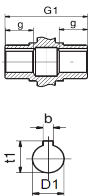
Output Hub
