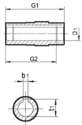
Output Hub
