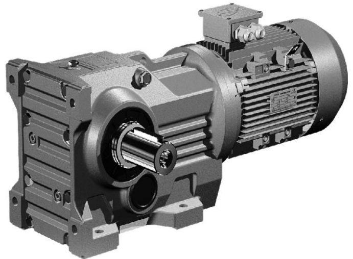
WK... FOOT MOUNTED BEVEL HELICAL GEARED MOTOR
