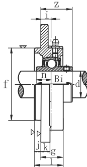
SR type seal
